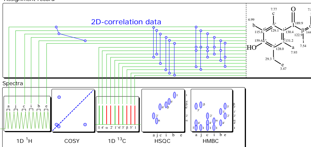
Computer-readable graphical description of proton, carbon, COSY, HMQC and HMBC, for some simple coupling systems of compound 2, José A. Bravo et José L. Vila, pp. 104-114
